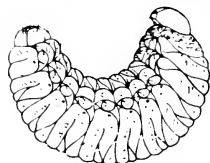
Fig. 76. Large Chestnut weevil, Curculio proboscideus Fab. (U.S.D.A.)
